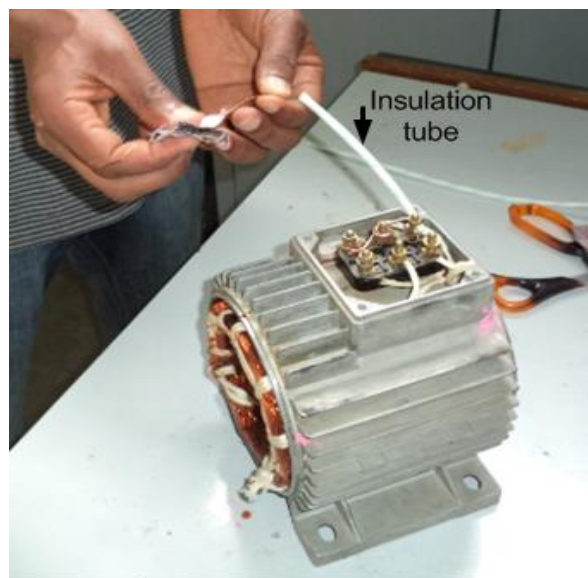
Figure 3.6 tube insertion
