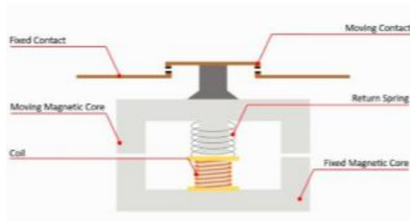
Figure 2.3 structure of contactor
