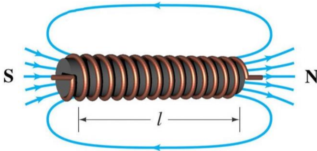
Figure 2.2 solenoid coil
