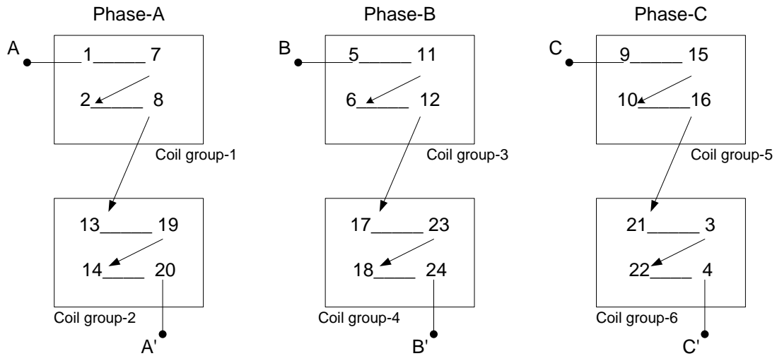
Figure 1.18 Connection diagram
