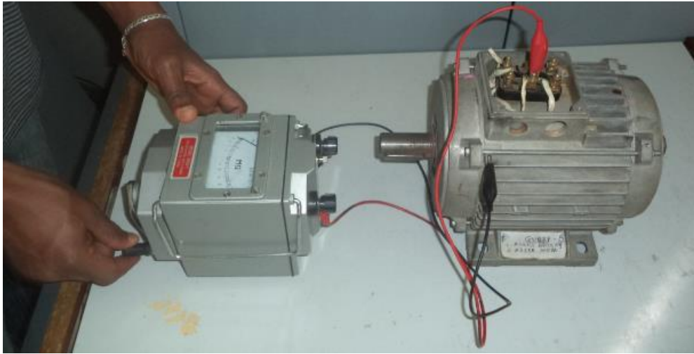
Figure 3.12 insulation resistance testing
