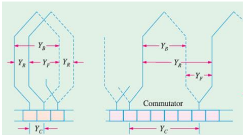
Figure 1.7 Pitch
