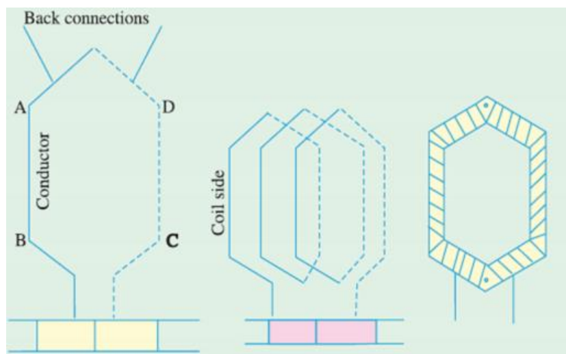
Figure 1.6 Conductors
