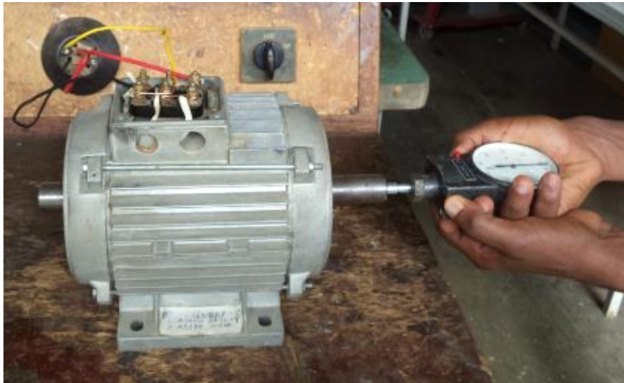
Figure 3.13 speed measurement
