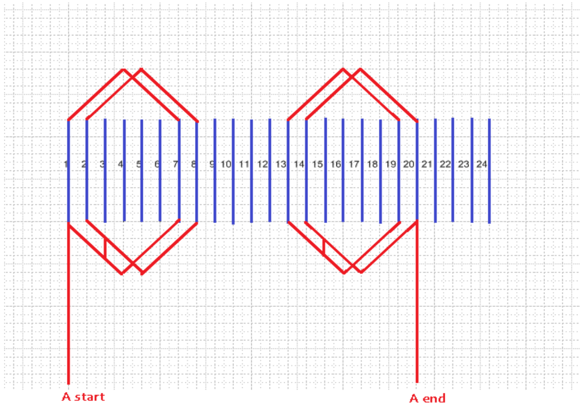
Figure 1.41 coil laying
