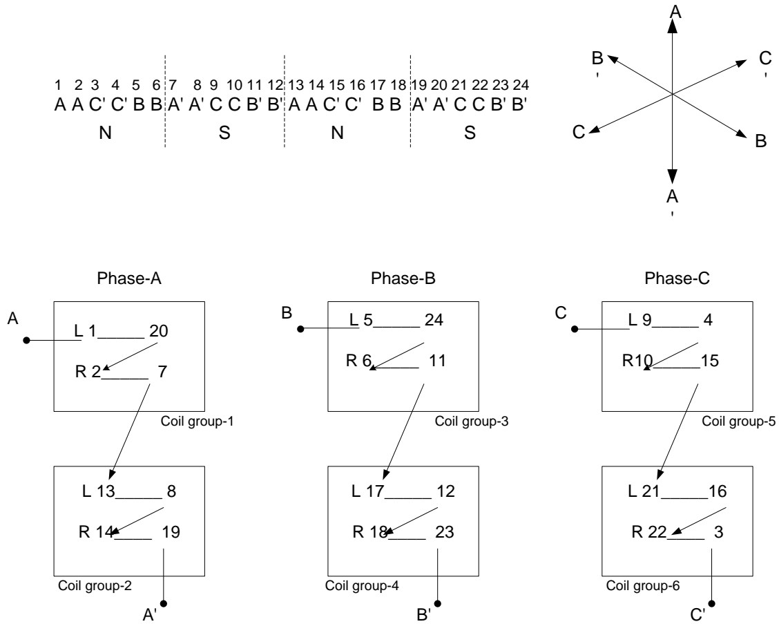
Figure 1.16 Connection diagram
