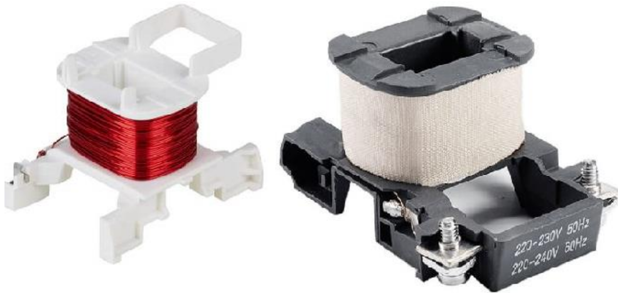
Figure 2.5 contactor winding
